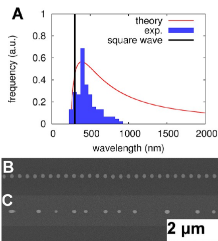
Figure 2. (a) The dispersion curve obtained based on the RP instability mechanism ((red) solid curve), along with the distribution of particle spacing obtained using line with a square wave perturbation of A_p = 295.8 \pm 5 nm, w_p = 112 \pm 5 nm, w = 112 \pm 5 nm, \lambda = 300 nm, and a thickness of 7 \pm 1 nm. (b-c) SEM images of the resulting particles from the square wave perturbed line and the unperturbed line of equivalent volume.
